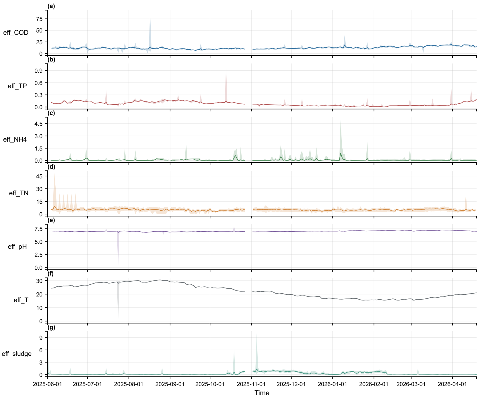
Effluent water-quality variables — full-span overview (daily min–max envelope) [2025-06-01~2026-04-19]
